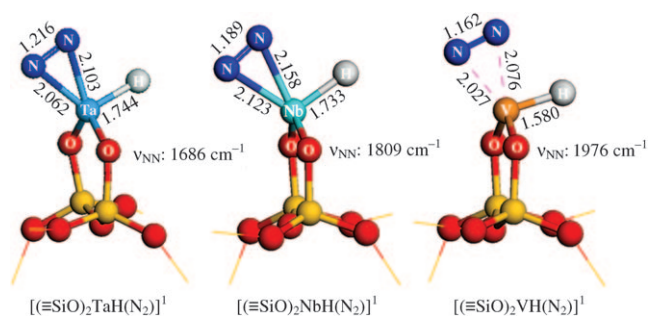
Figure 4. Optimized geometries of [(\text{SiO})_2\text{TaH}(\text{N}_2)]^+ , [(\text{SiO})_2\text{NbH}(\text{N}_2)]^+ , and [(\text{SiO})_2\text{VH}(\text{N}_2)]^+ with bond lengths [ \text{\AA} ].
